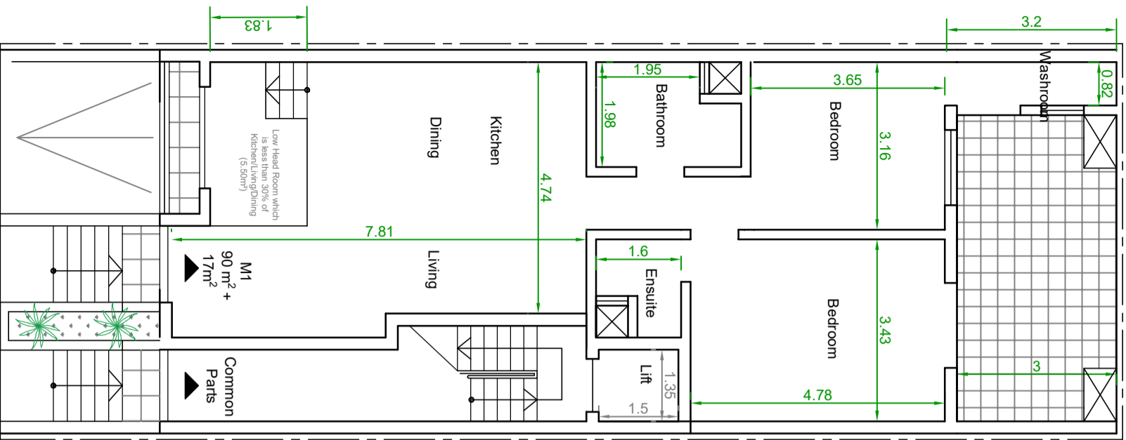
Ground Floor
