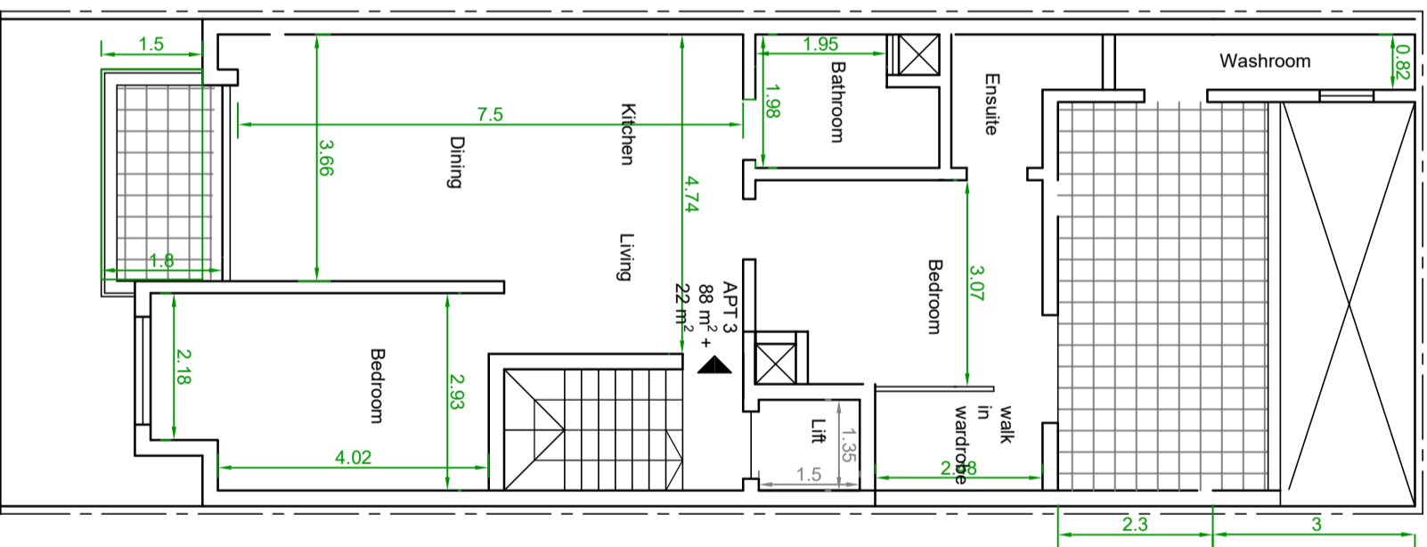
Third Floor
